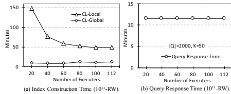
Fig. 12. Scalability with Increasing Number of Executors.
