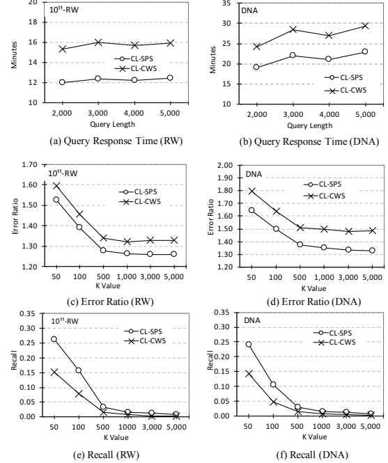
Fig. 9. Query Evaluation (CL-SPS vs. CL-CWS).
