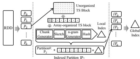
Fig. 1. Two-level Indexing Strategy in ChainLink.
