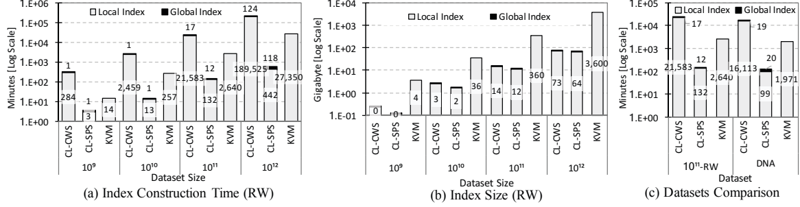
Fig. 7. Index Construction Analysis [Log Scale].
