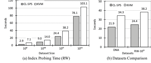
Fig. 11. Query Evaluation (CL-SPS vs. KVM).
