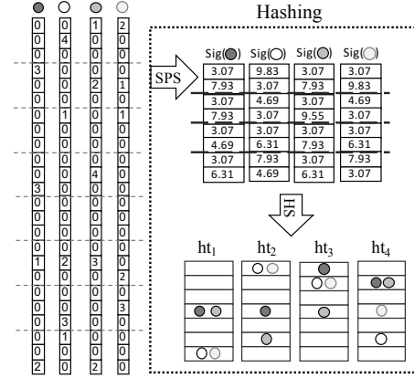
Fig. 4. Hashing Weighted Sets Using Algorithm 1 Single Pass Signature (SPS) Followed by Hashing Signatures (HS) using Algorithm 2.
